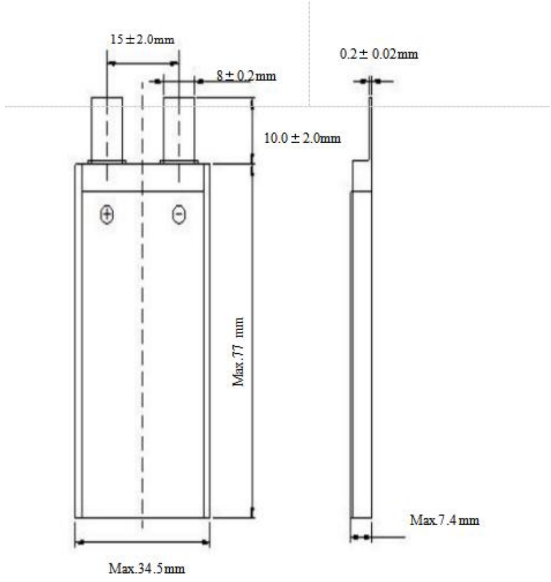
Fig.1 Dimensional Drawing of 743476-40C-1600mAh
