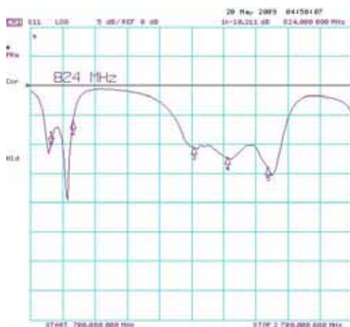
- Return loss -
