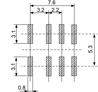
Recommended mounting pad (Tolerance: ±0.1mm)
