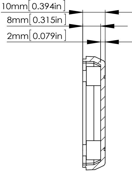
SECTION B-B SCALE 1 : 1
