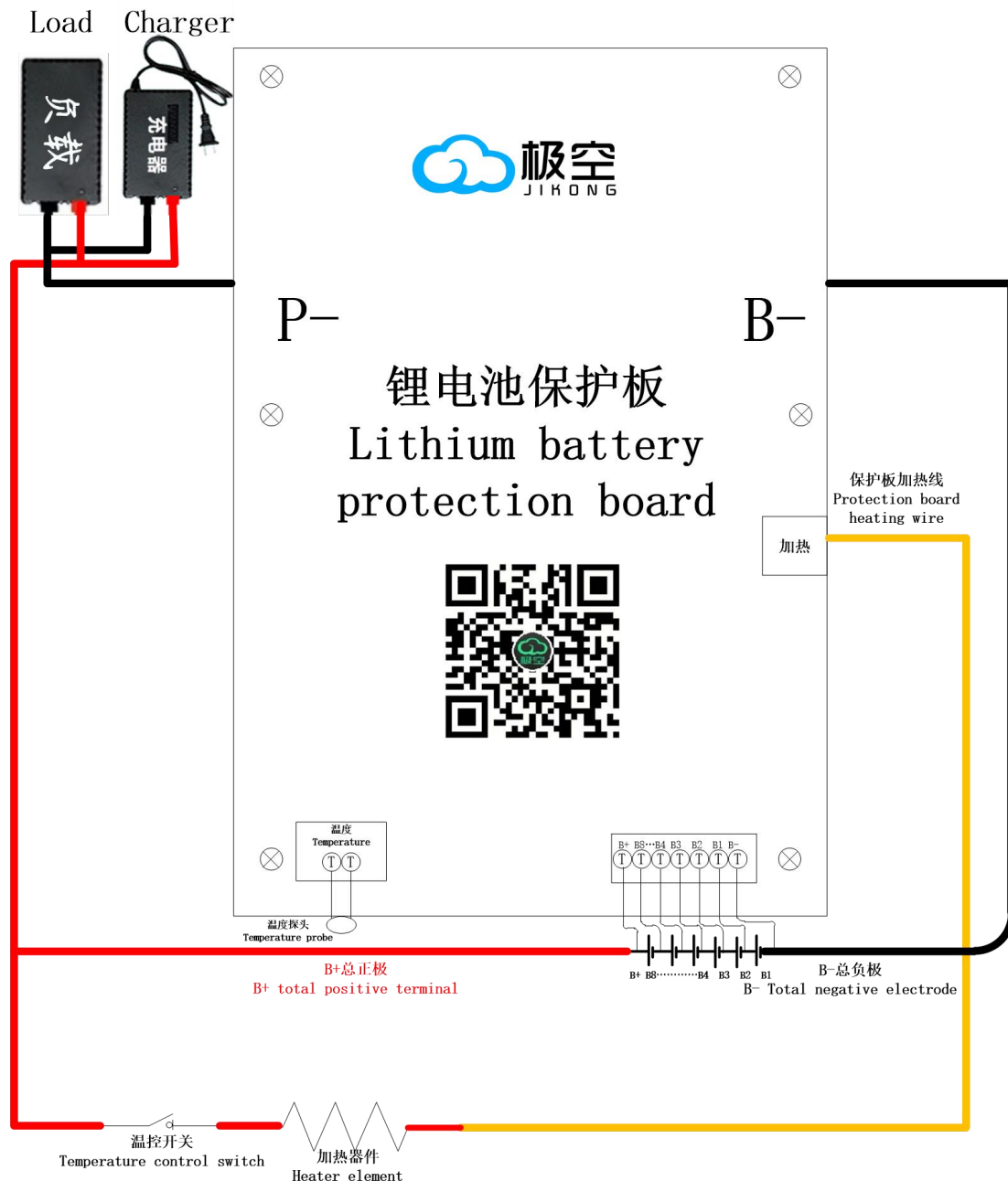
JK-B1A8S-10PS接线图
