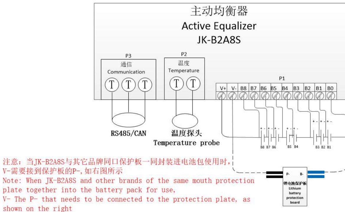
JK-B2A8S 接线图 JK-B2A8S wiring diagram
