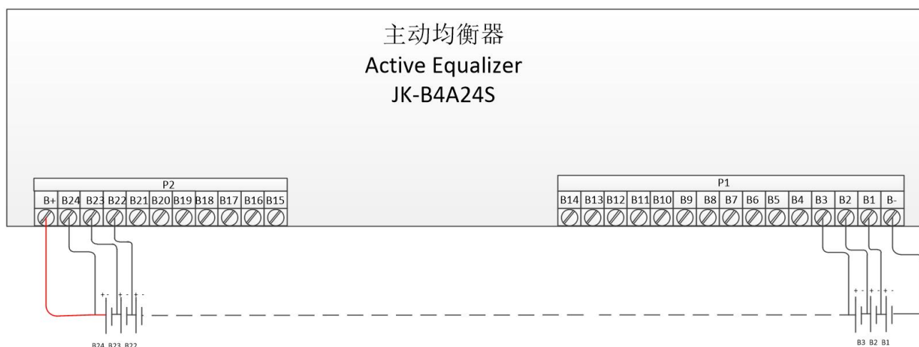
JK-B4A24S 接线图 JK-B4A24S wiring diagram
