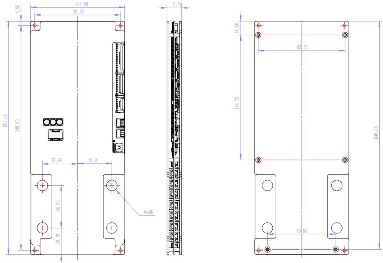
JK-BD6A32S-10P/15P外形尺寸
