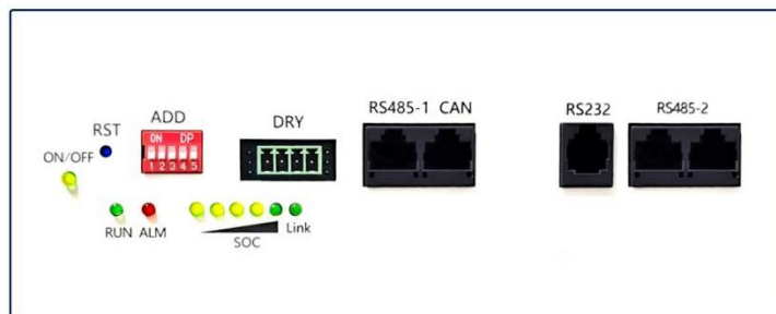
从机地址1设置示例(Example of Setting Slave Address 1)
