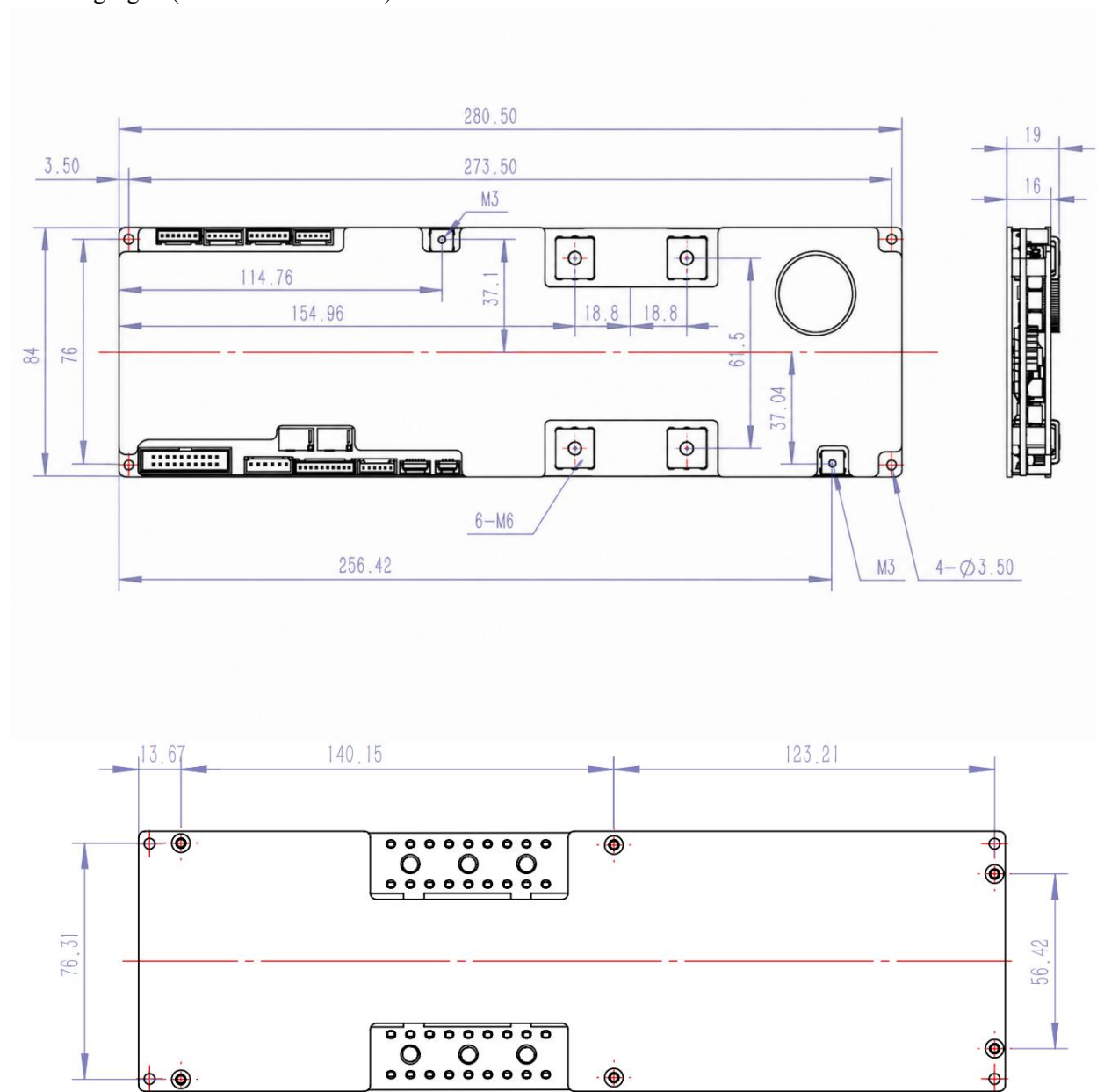
JK-PBD6A16S-20P 外形尺寸
