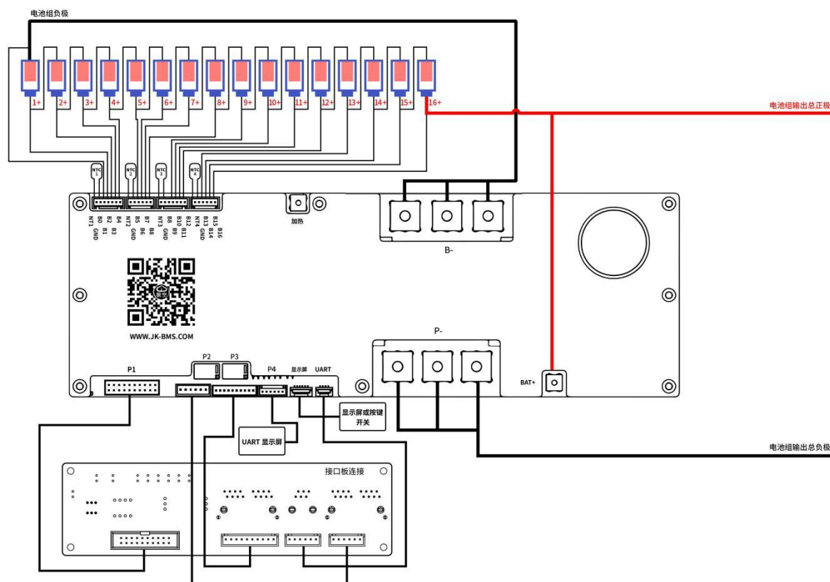
JK-PBD6A16S-20P 接线图
