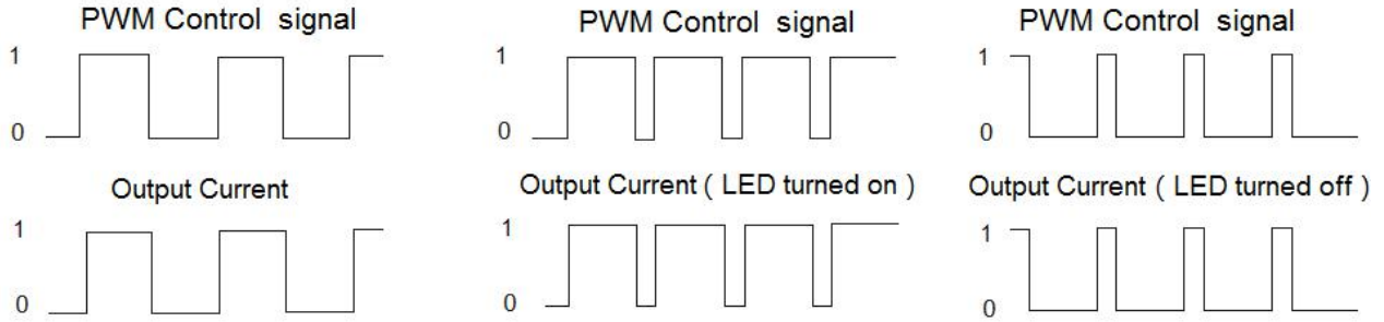
Fig. 4 PWM Dimming control
