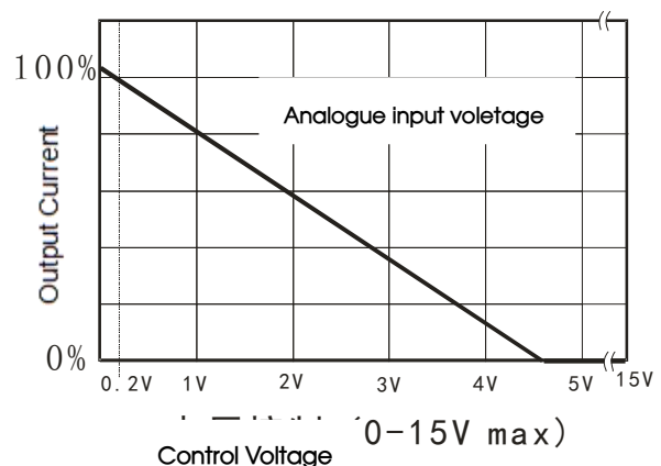
Fig. 7 Analogue input voltage and output current
