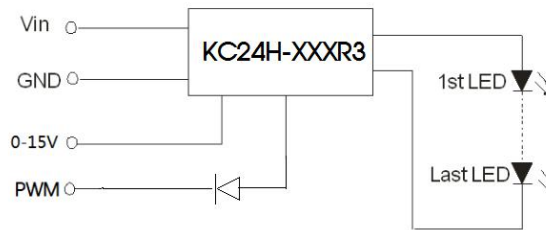
Fig. 5 PWM Dimming control circuit diagram
