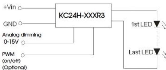
Fig. 6 Analogue Dimming circuit diagram
