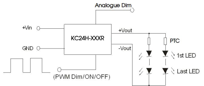
Fig. 3 Parallel application
