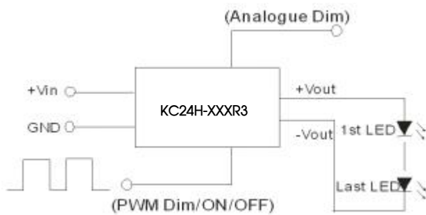
Fig. 2 Series application
