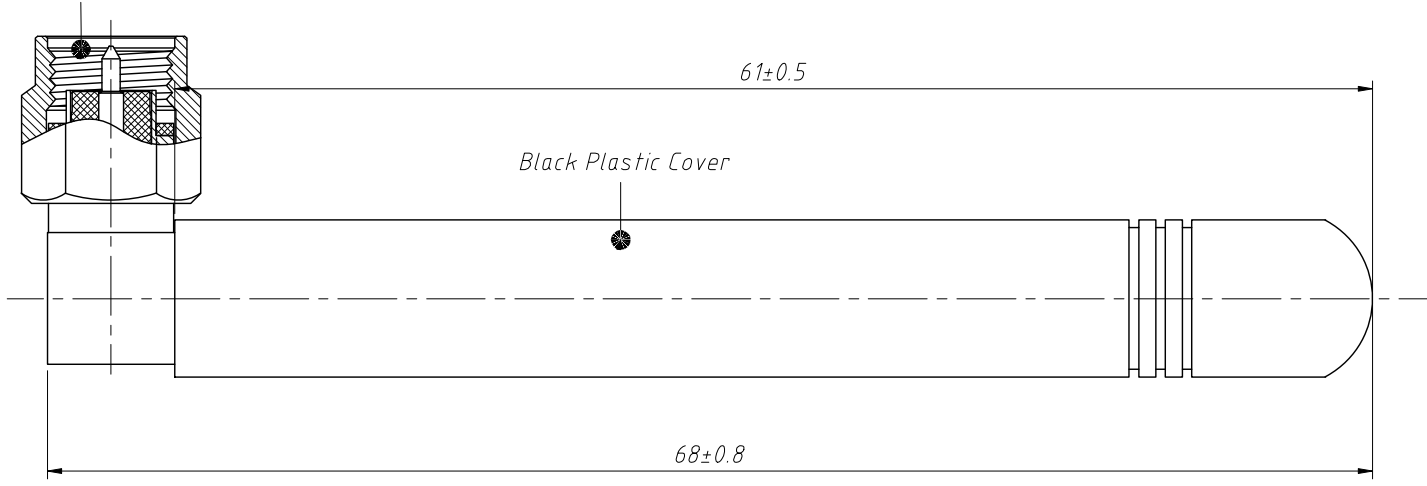
SMA Male Connector
