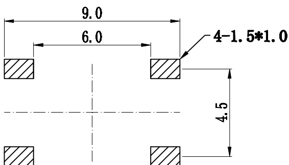
PCB线路板安装图(±0.1) PCB Layout Drawing (±0.1)
