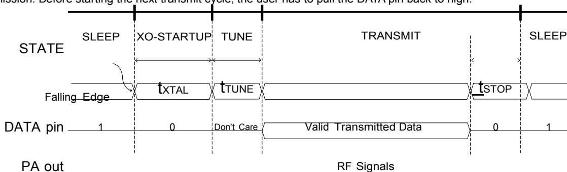
Figure 12. Transmission Enabled by DATA Pin Falling Edge
