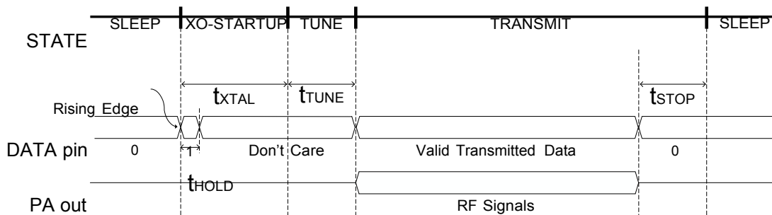
Figure 11. Transmission Enabled by DATA Pin Rising Edge
