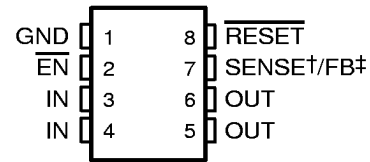
PW PACKAGE (TOP VIEW)
