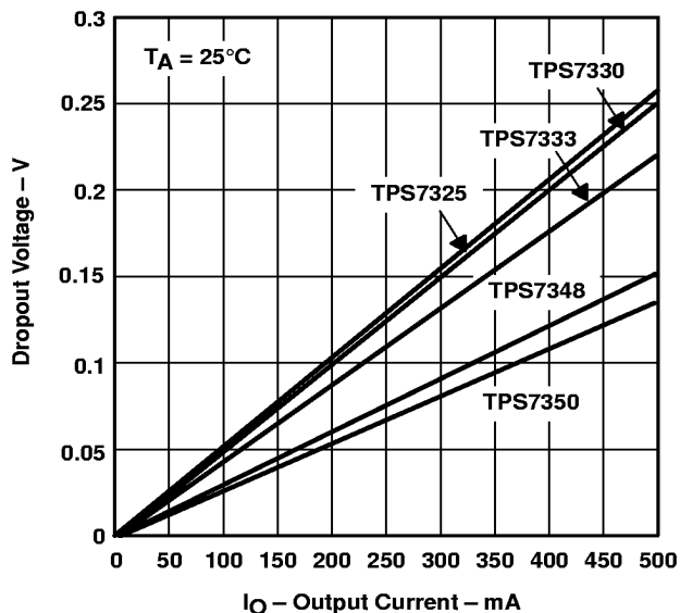
Figure 1. Dropout Voltage Versus Output Current
