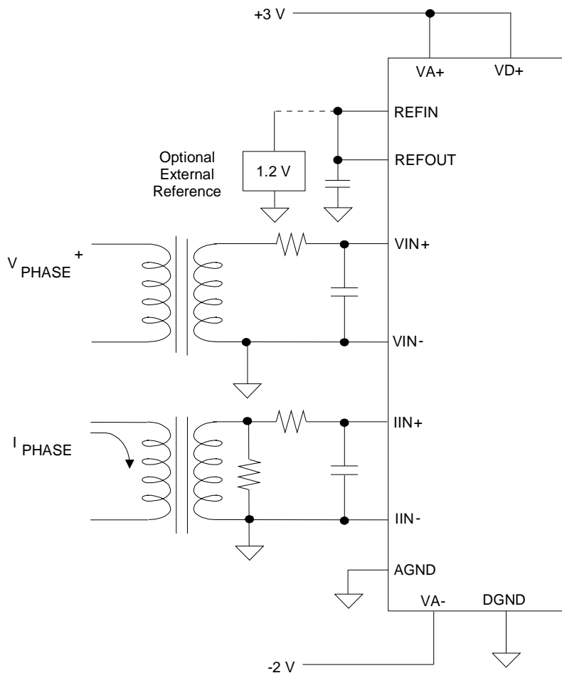
Figure 2. Typical Connection Diagram
