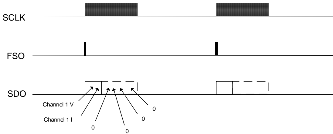
Figure 3. Serial Port Data Transfer
