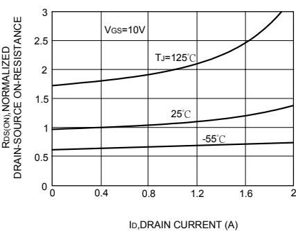
Figure 4. On-Resistance Variation with Drain Current and Temperature
