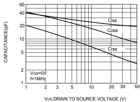
Figure9.Capacitance Characteristics
