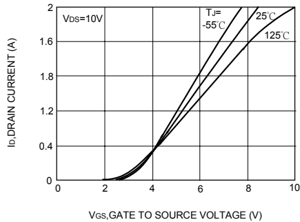
Figure 5. Transfer Characteristics
