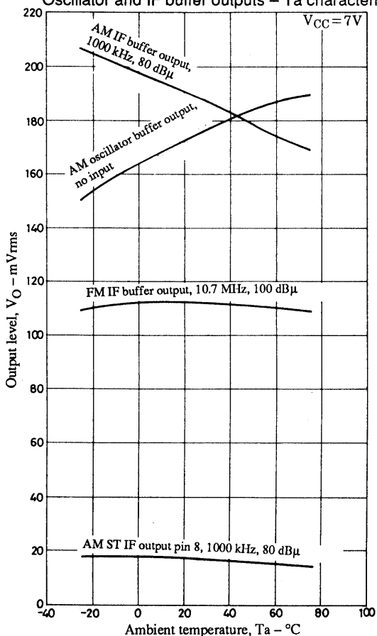
Oscillator and IF buffer outputs - T_a characteristics
