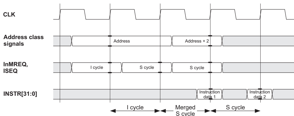
Figure 4-4 Merged I-S cycle
