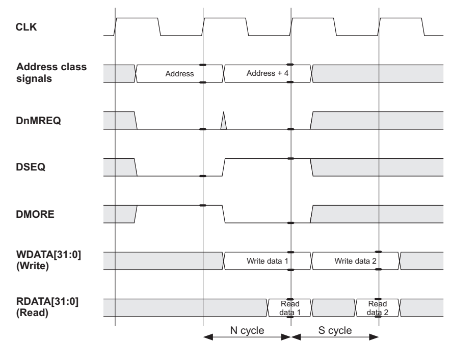
Figure 4-11 Sequential access cycles
