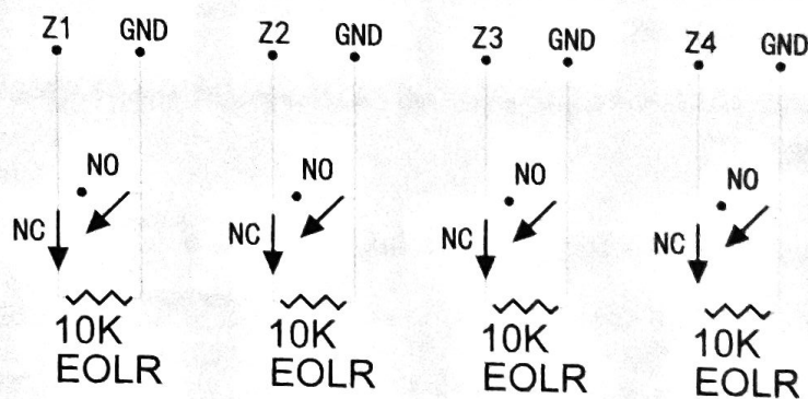
the Hardwired Zones Connections Diagram
