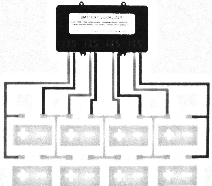
8x12V Battery
