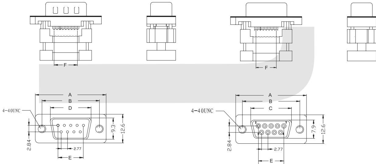
Dimension
