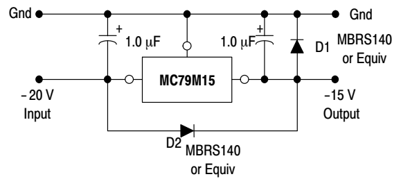
Figure 2. Protection Diodes
