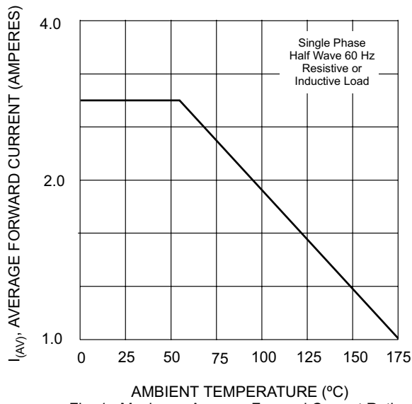
Fig. 1, Maximum Average Forward Current Rating
