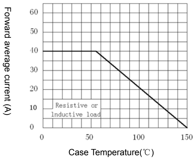
Forward av. current decrease curve
